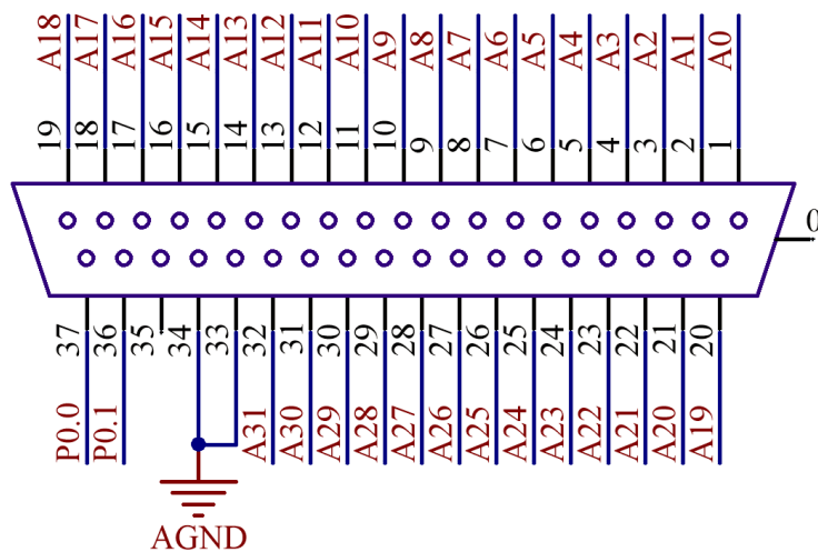
PD32 Signals
