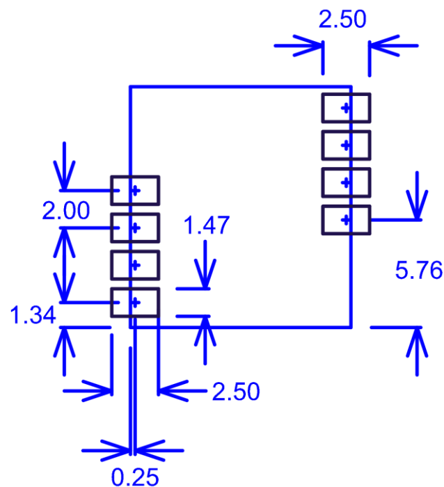
Figure 7. PCB Footprint (mm)
