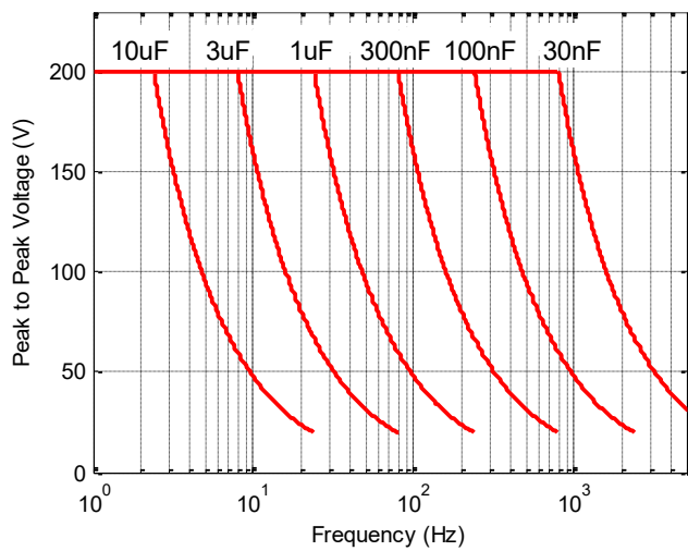
Figure 4. Power bandwidth
