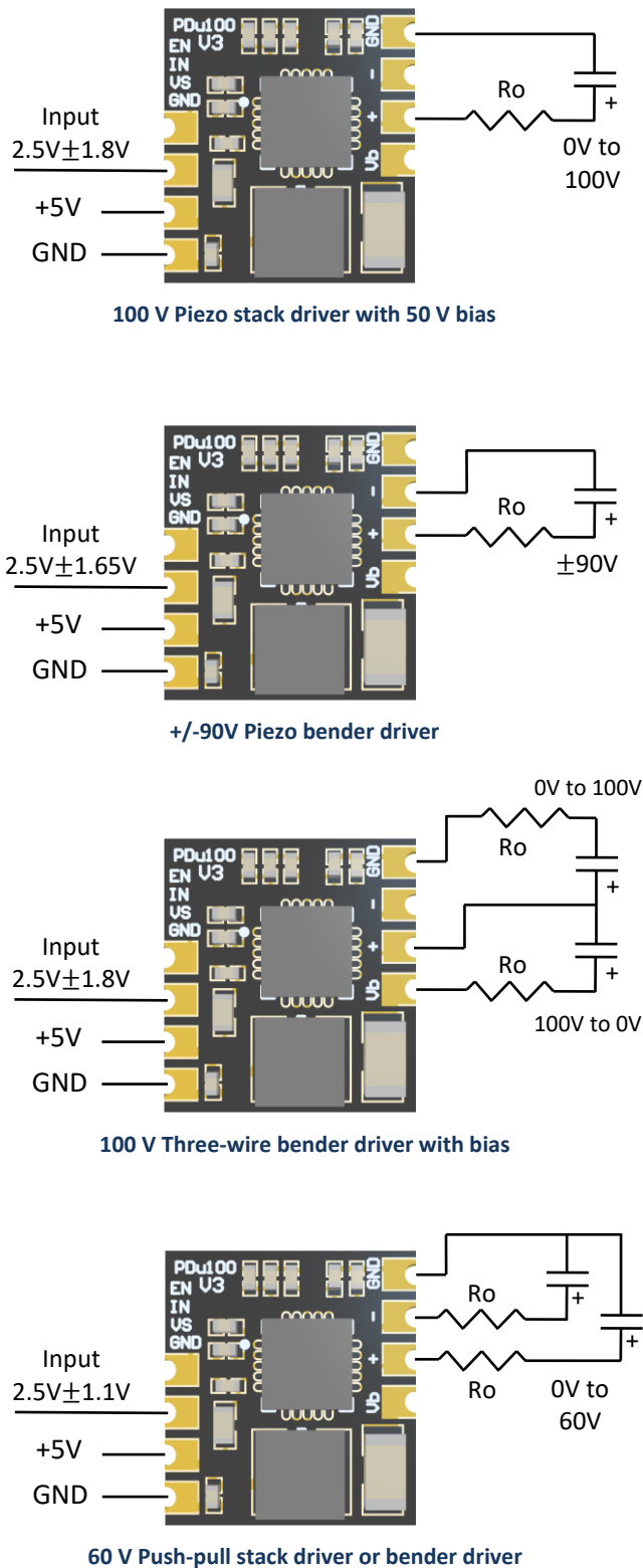
Figure 3. Application circuits
