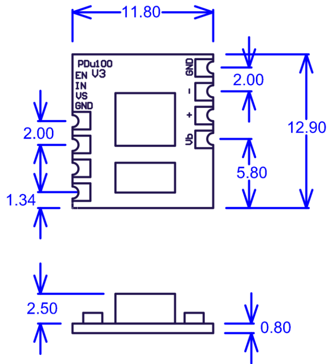
Figure 6. Dimensions (mm)
